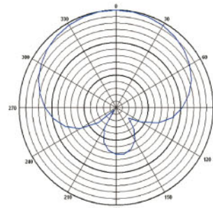
Measure Distance - 50 cm Test Instrumental - Bruel & Kjaer 2012 & 9640
